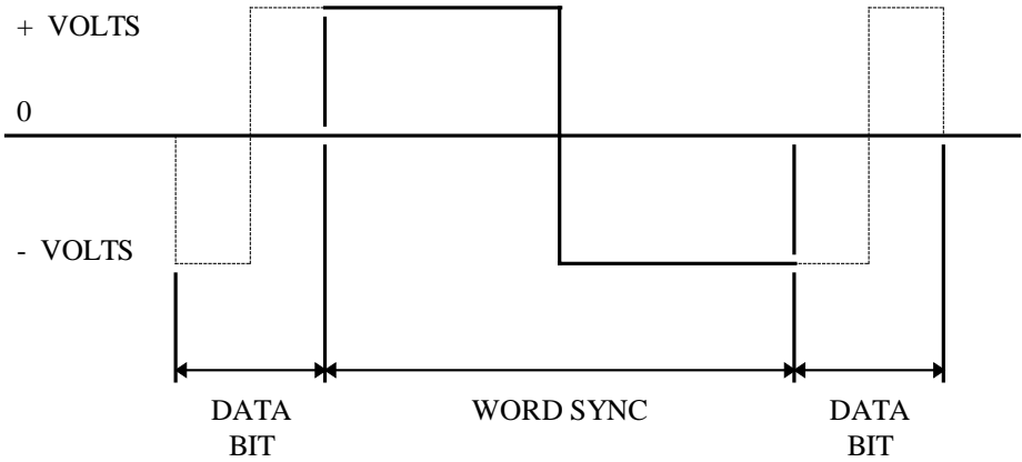
FIGURE 4. Command and Status Sync
