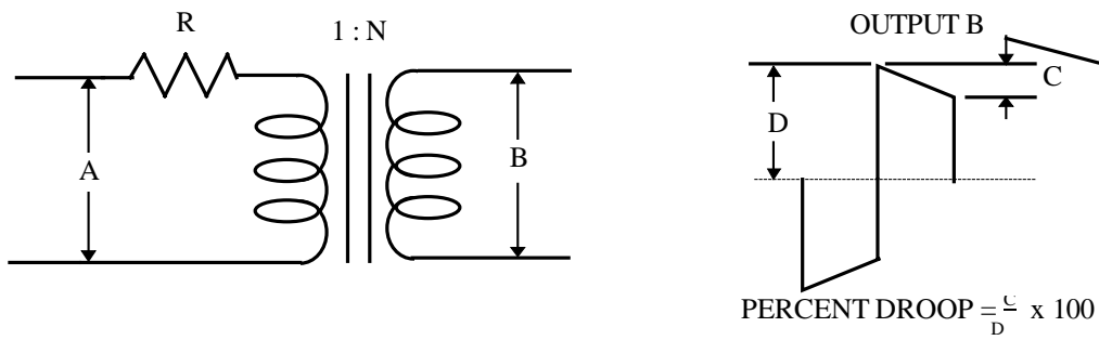
FIGURE 11. Coupling Transformer
