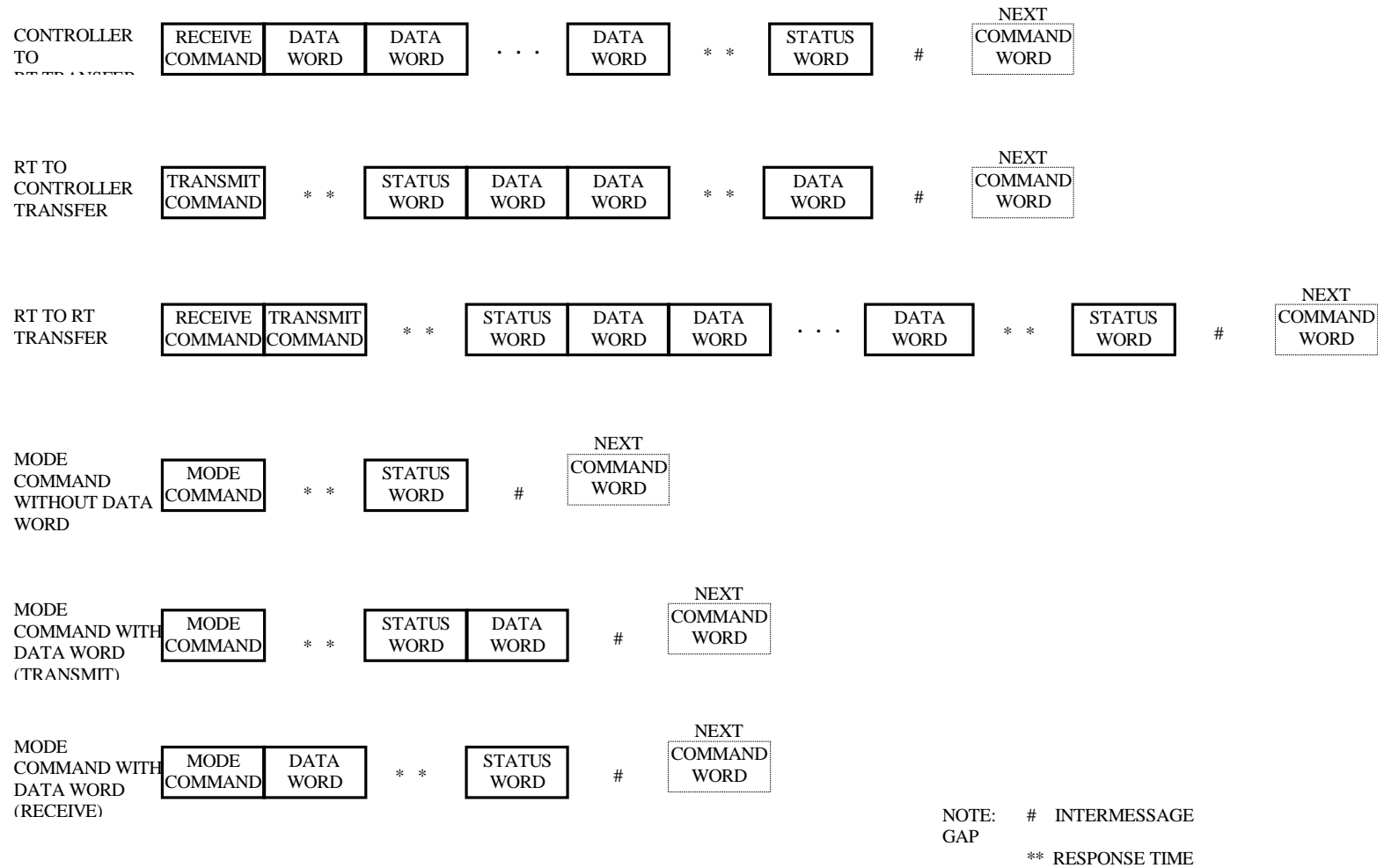
FIGURE 6. Information Transfer Formats
