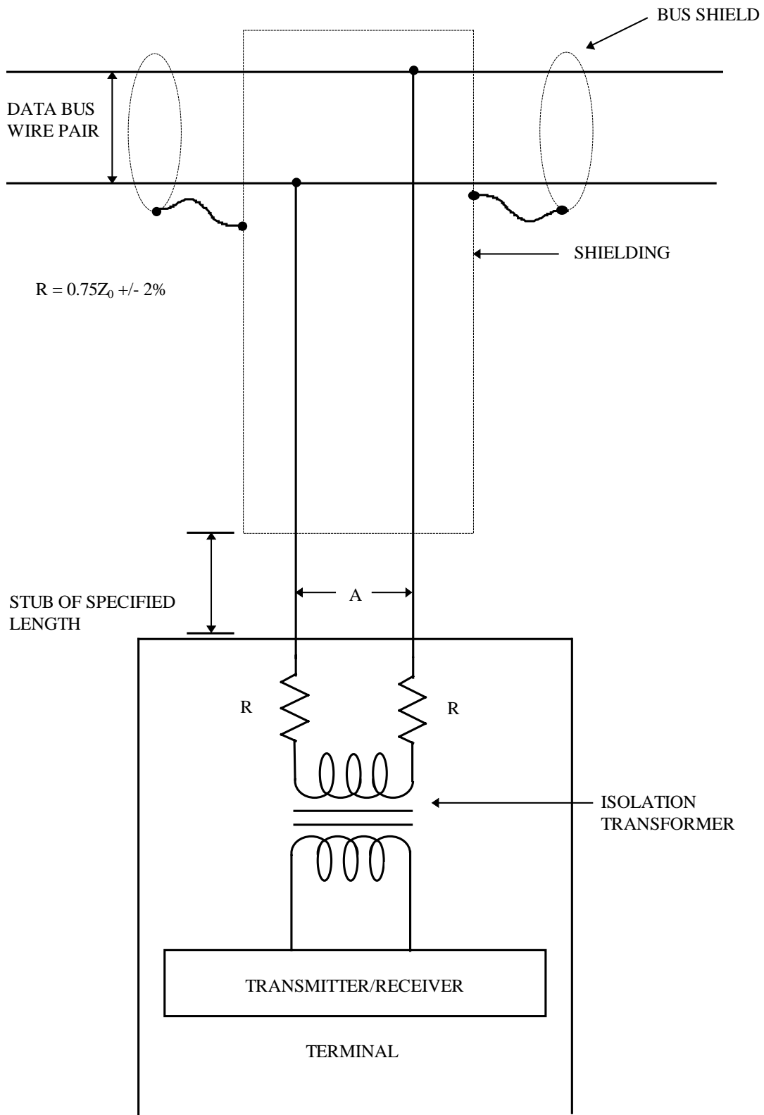
FIGURE 10. Data Bus Interface Using Direct Coupling
