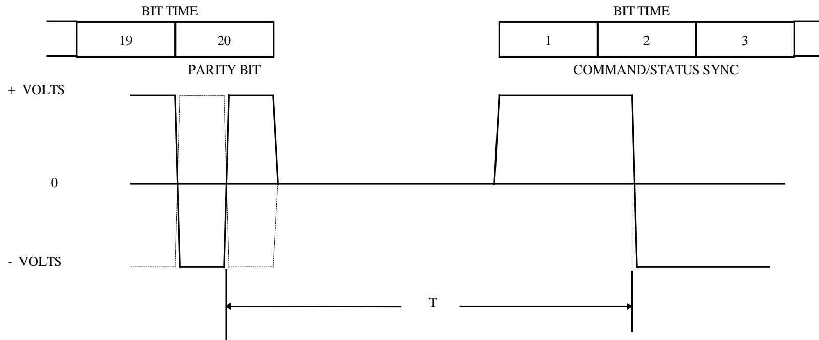
FIGURE 8. Intermessage Gap and Response Time
