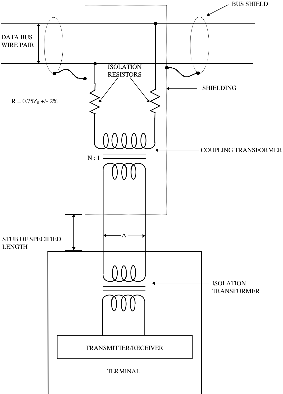
FIGURE 9. Data Bus Interface Using Transformer Coupling
