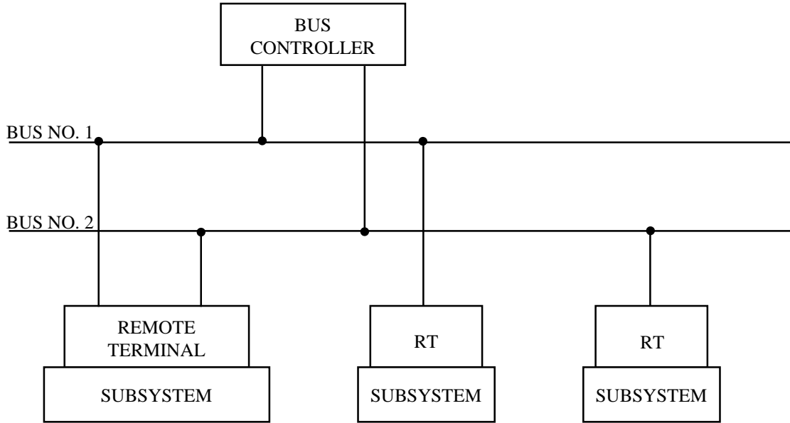
FIGURE 10.1. Illustration of Possible Redundancy
